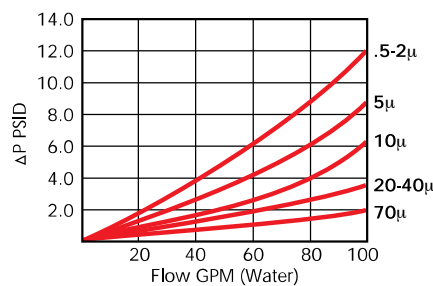
Flow Rate Vs. \Delta P
